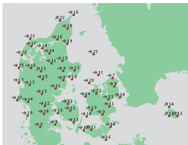
Middelvind (m/s) 14. jan 2007 05:40
